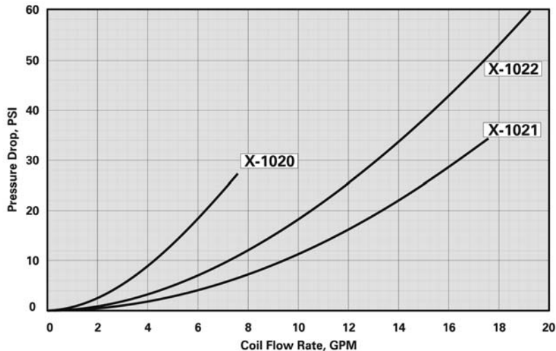
Figure 11.1: Tankless Coil Pressure Drops
